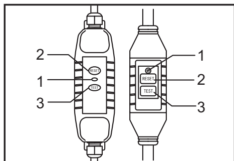
► 1. Pilot lamp 2. RESET (R) button 3. TEST (T) button
